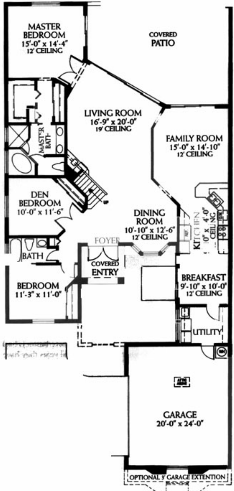
FIRST FLOOR
