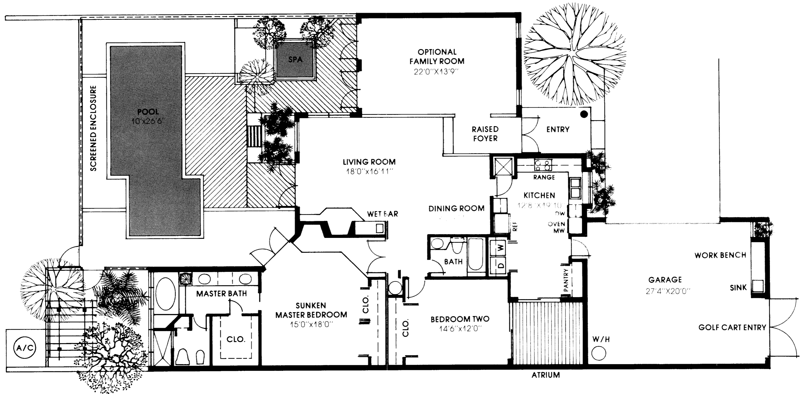
UNIT D FIRST FLOOR
