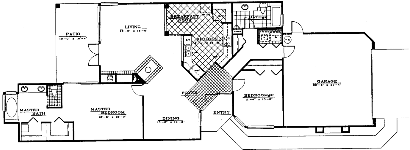
UNIT A - FLOOR PLAN
