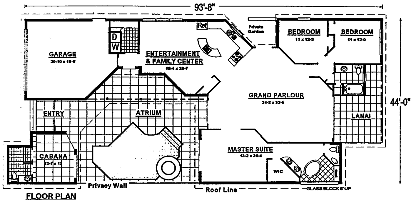
FLOOR PLAN
