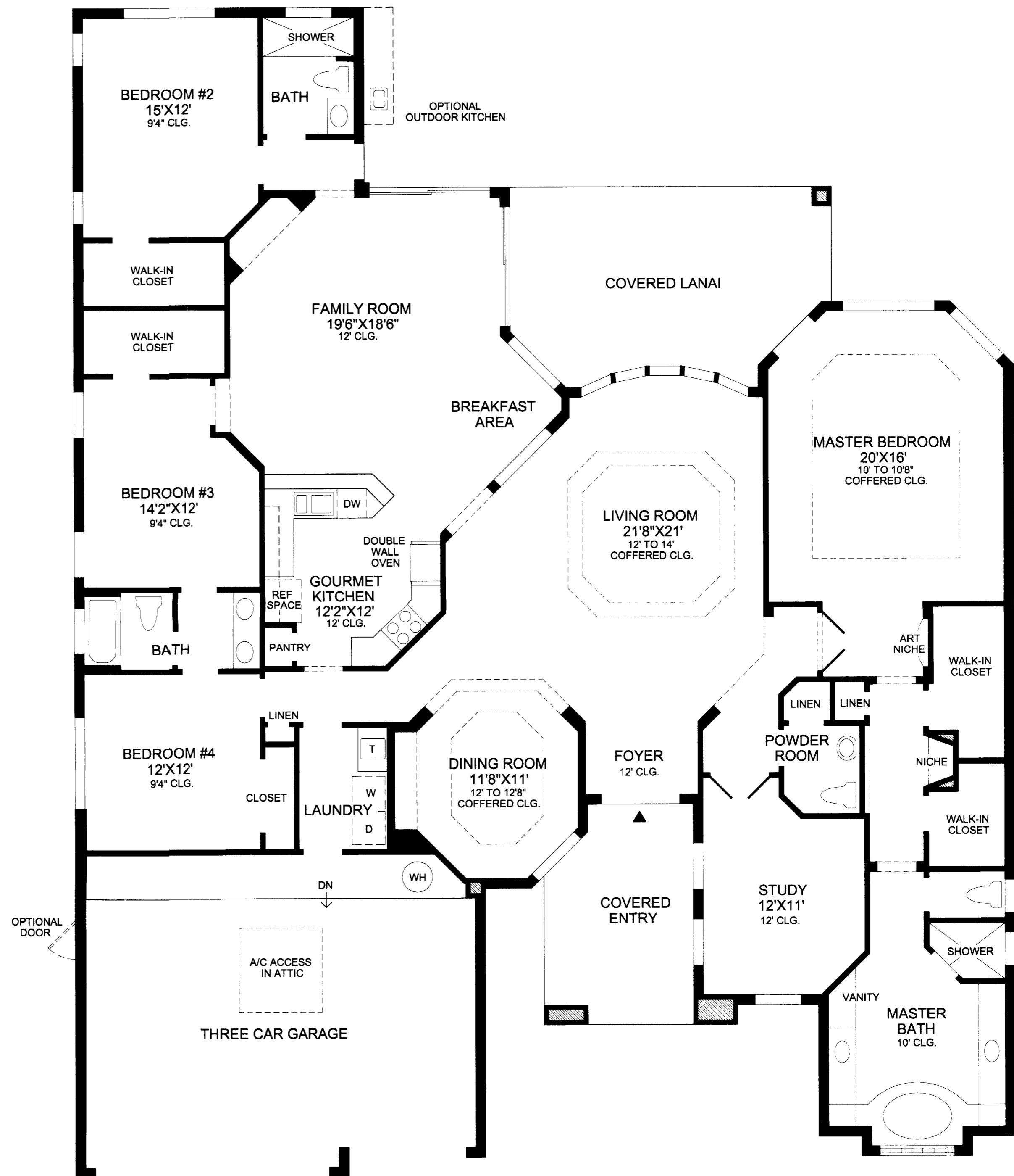
FLOOR PLAN
