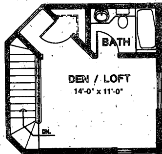
Second Floor Option C
