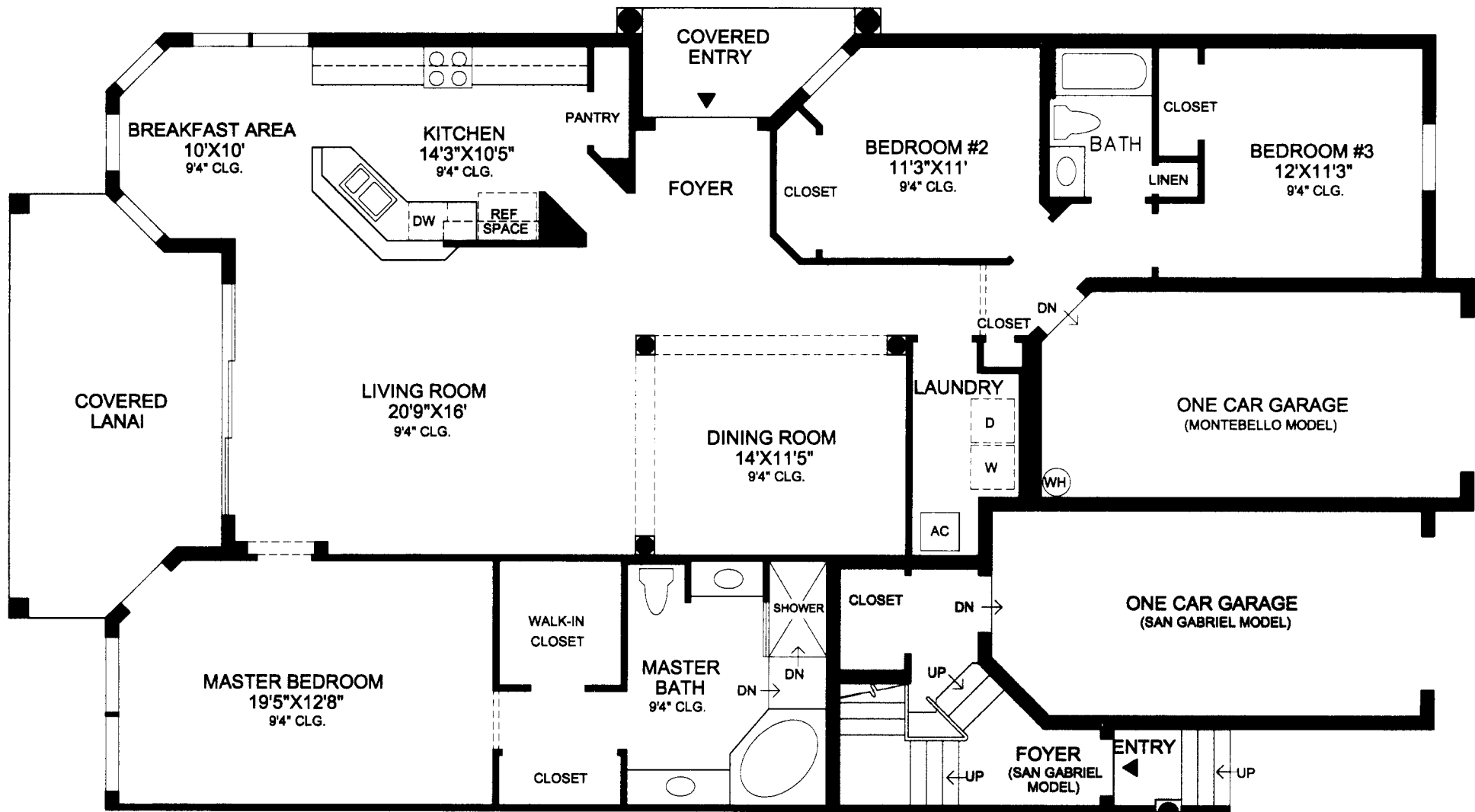
FIRST FLOOR LIVING UNIT
