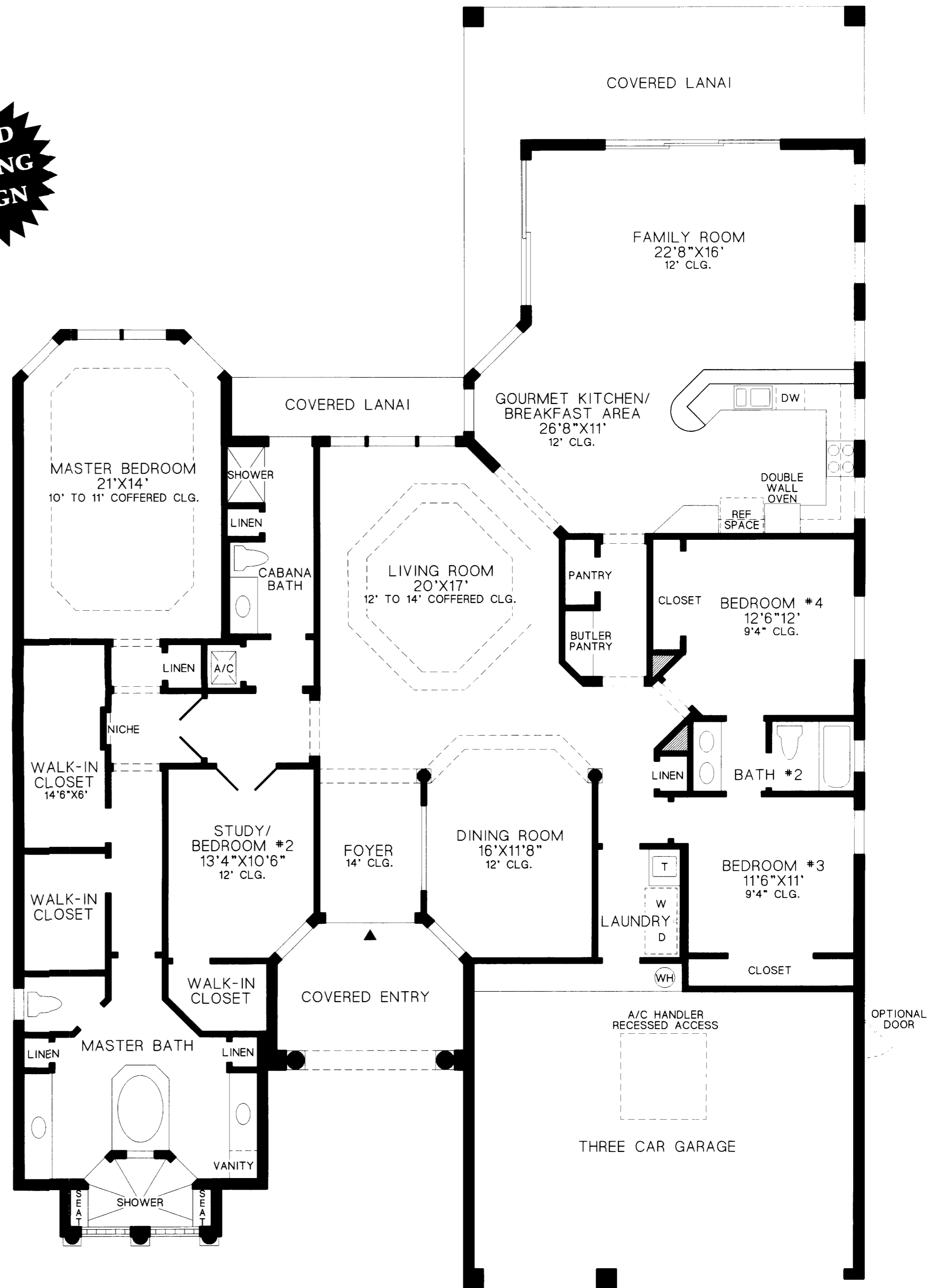
FLOOR PLAN
