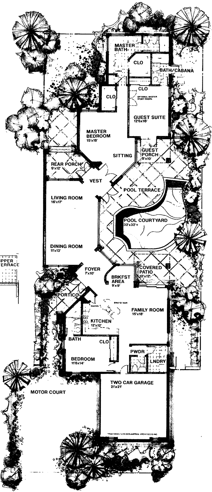
First Floor Plan with Stair Included
