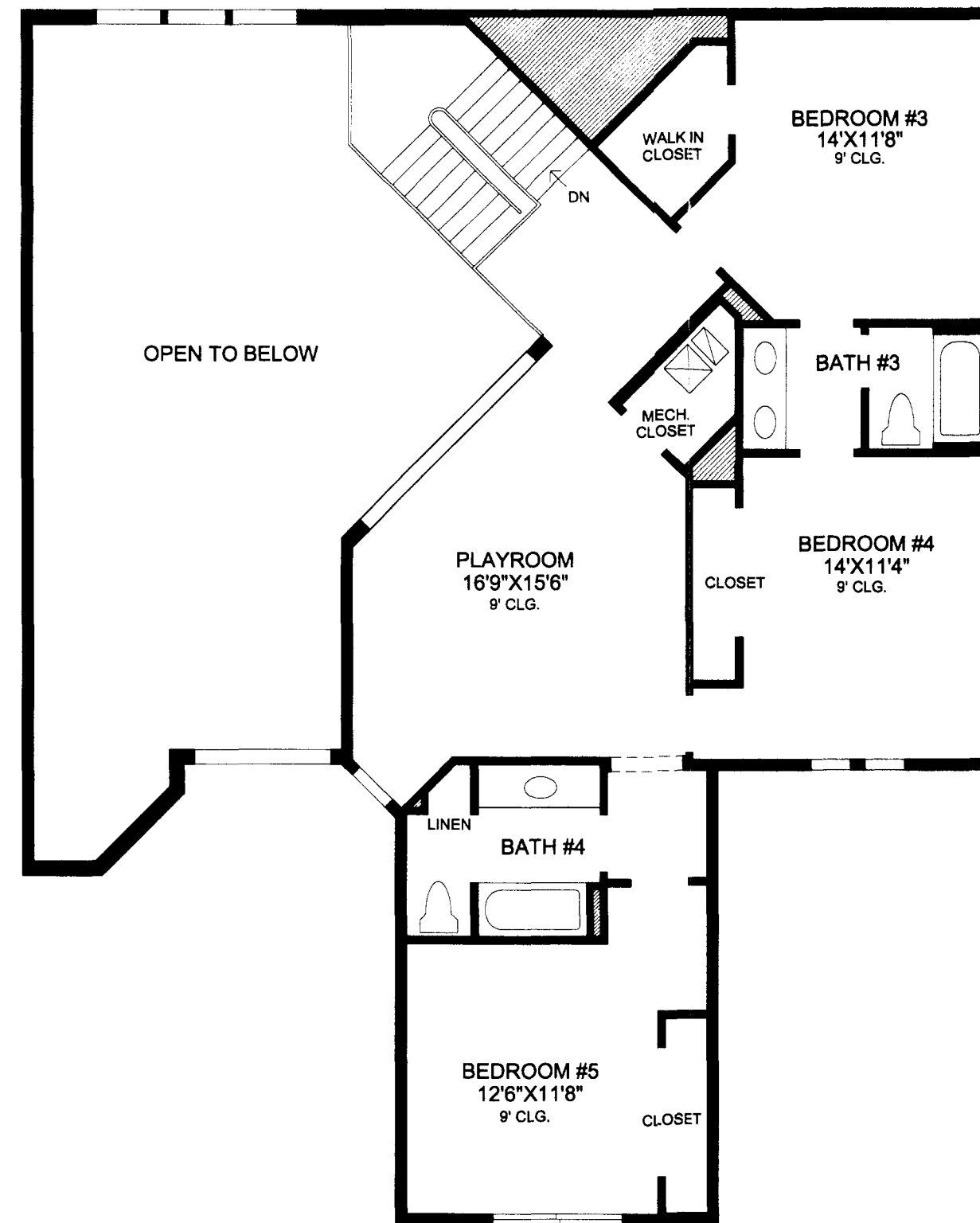
SECOND FLOOR
