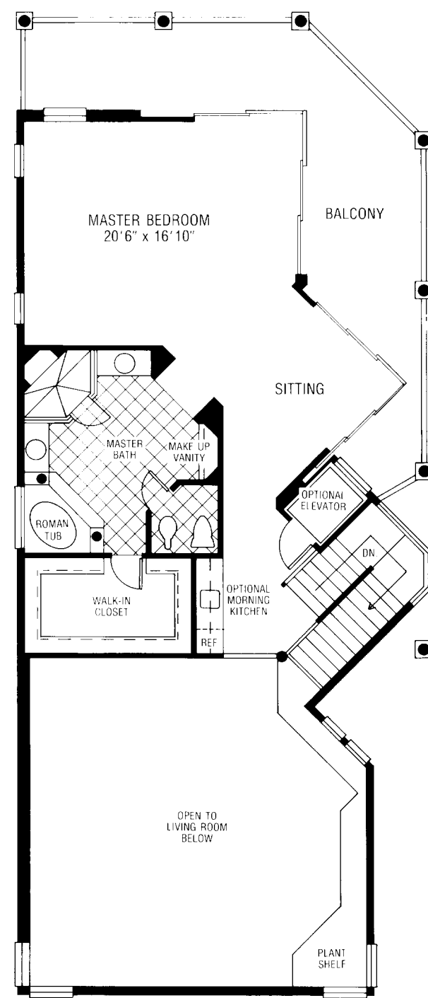
SECOND FLOOR
