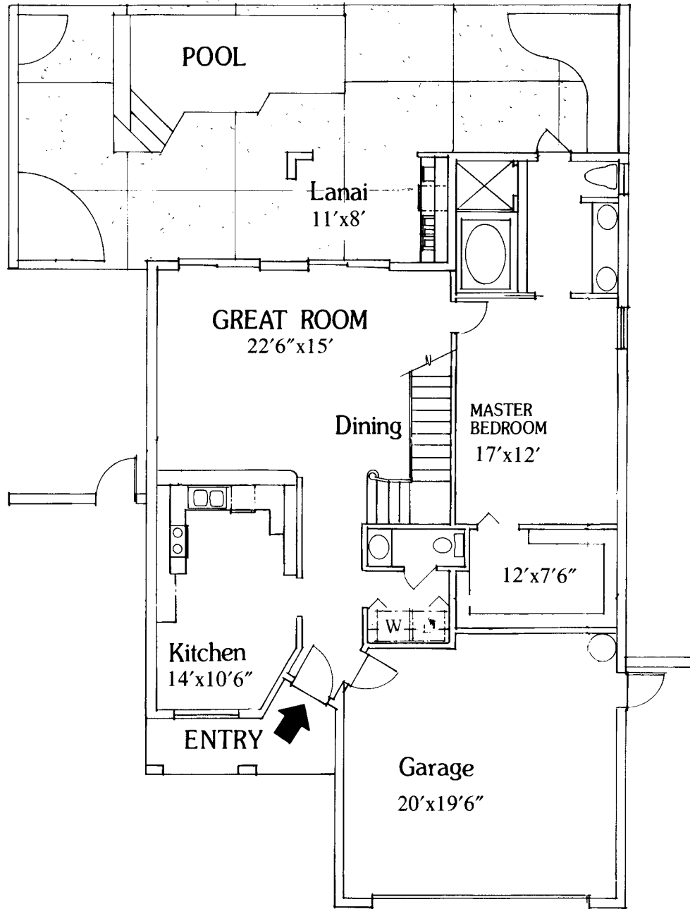
FIRST FLOOR
