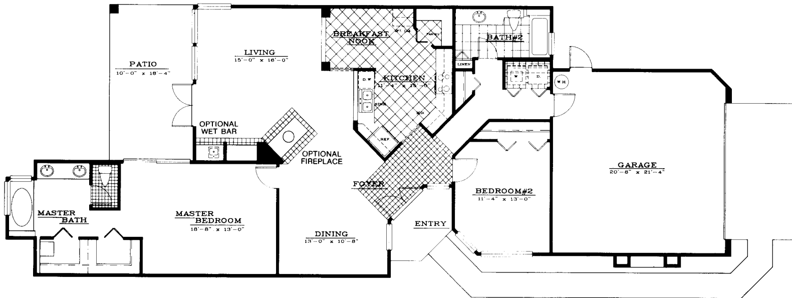
ALTERNATE GARAGE
