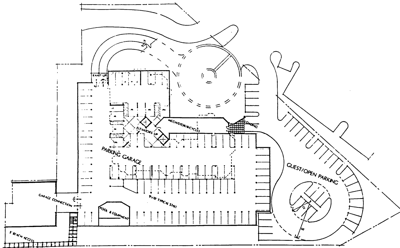
PARKING LEVEL PLAN
