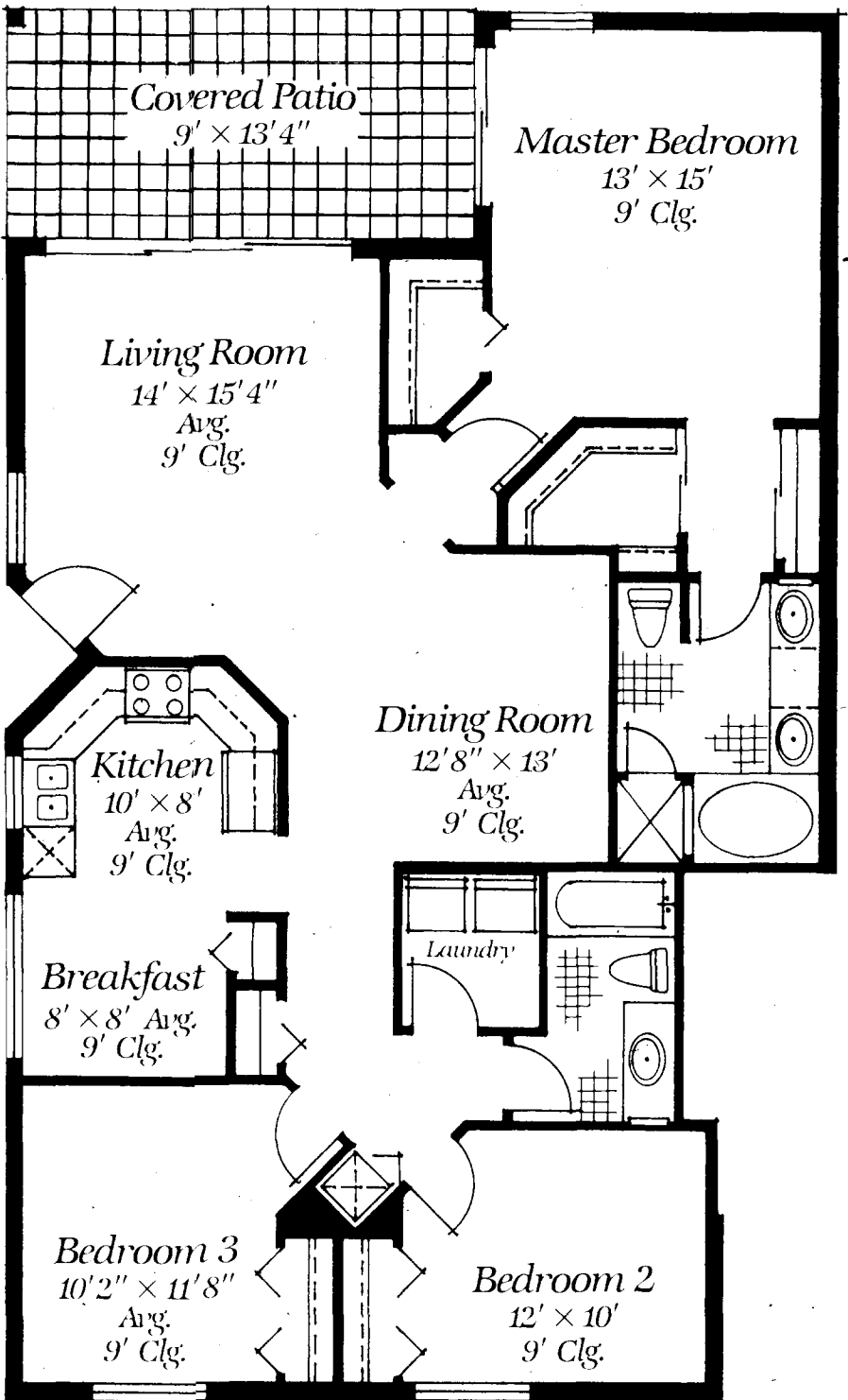
First Floor Three Bedroom Total Square Footage: 1,638
