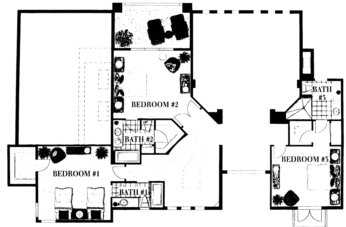
SECOND FLOOR
